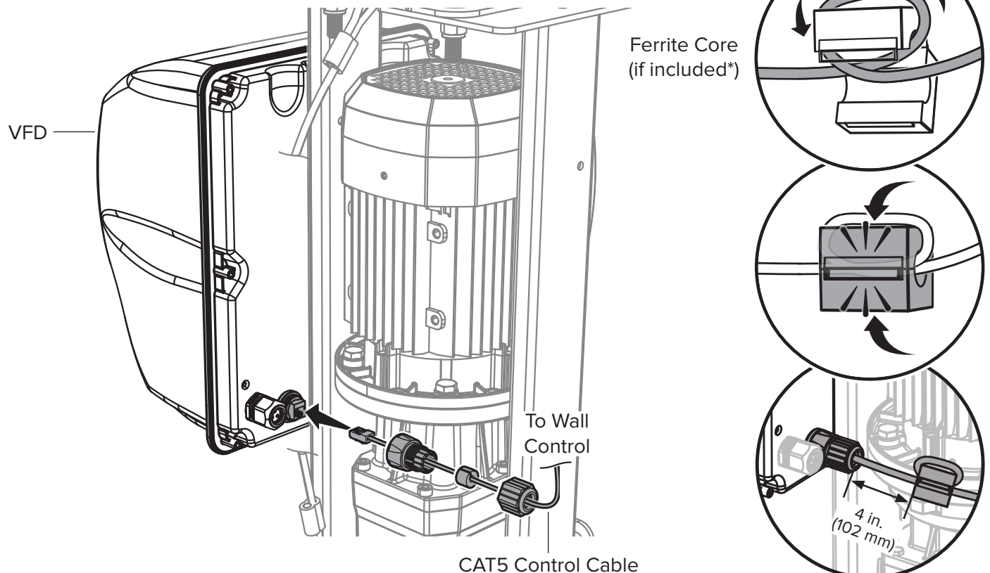
Fig. 1: CAT5 Control Cable to VFD
